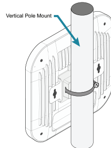
Figure 7. Vertical Pole Mounting of BSAP
