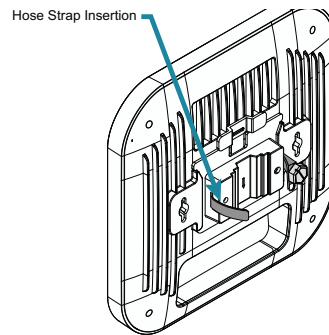
Figure 6. Attach the Pole Mounting Bracket for Vertical Mounting
