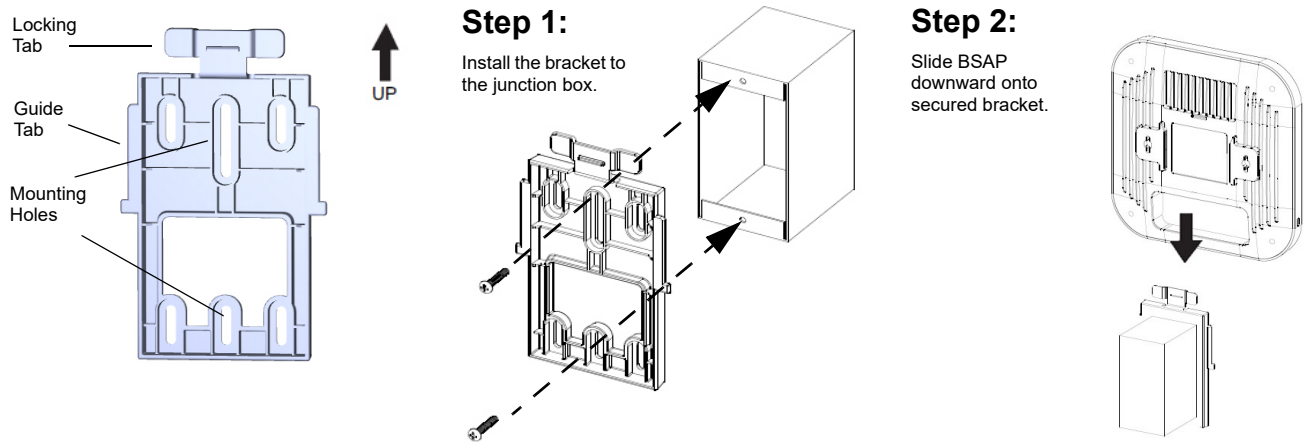
Figure 10. Mounting the BSAP to a Junction Box Bracket
