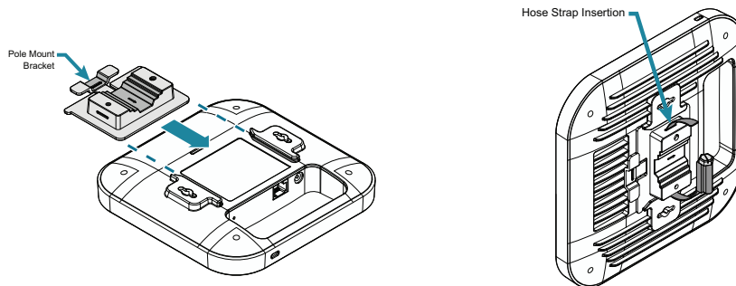
Figure 8. Attach the Pole Mounting Bracket and Straps for Horizontal Mounting
