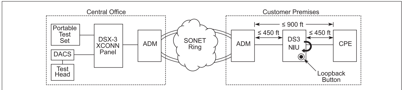
Figure 2. NIU3 Circuit Diagram
