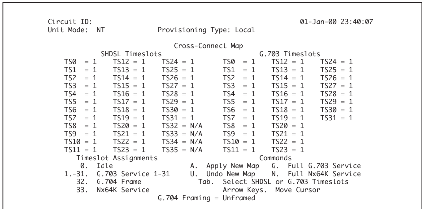
Figure 9. Unframed Full E1 Service
