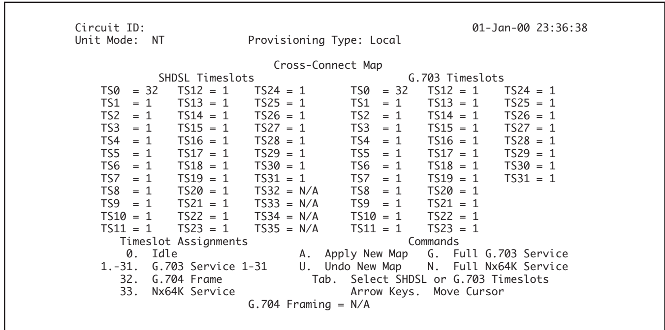
Figure 8. Framed Full E1 Service
