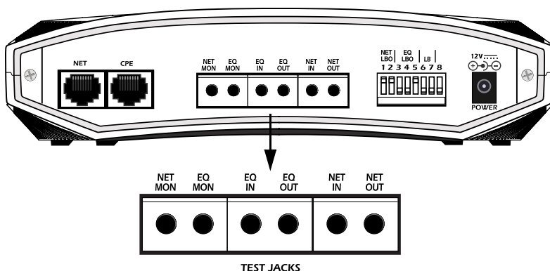
Figure 2-1. T1 CSU ACE Bantam Jacks
