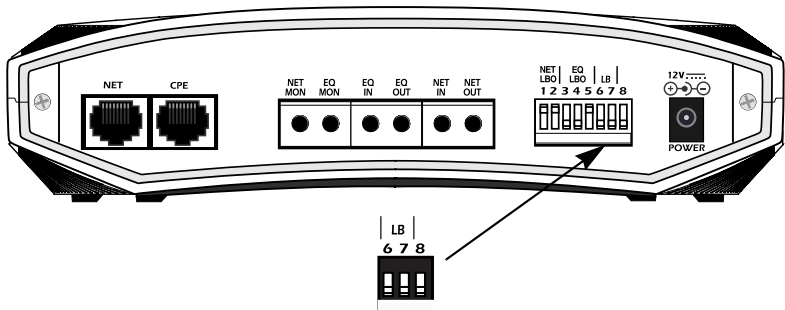
Figure 1-5. T1 CSU ACE Loopback Switch and LED
