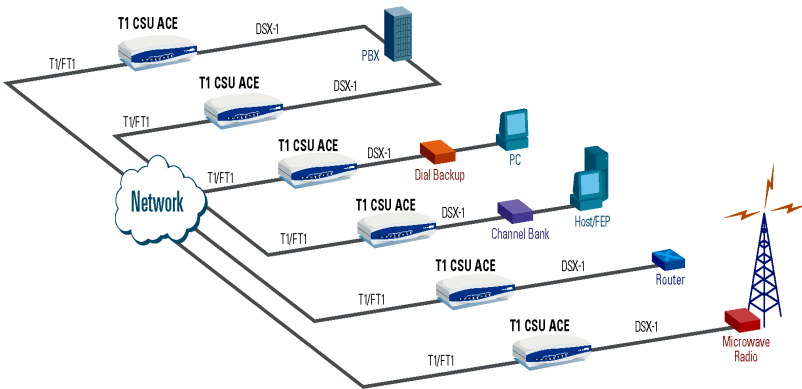
Figure 1-1. T1 CSU ACE Applications
