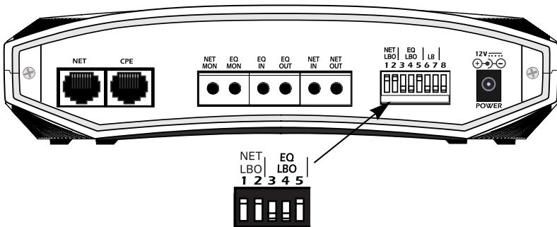
Figure 1-6. Line Build Out Switch
