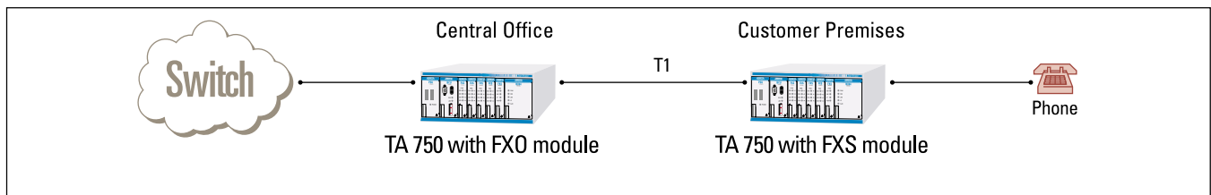
Figure 2. FXO to FXS Deployment
