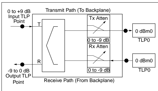
Figure 4. Circuit Path
