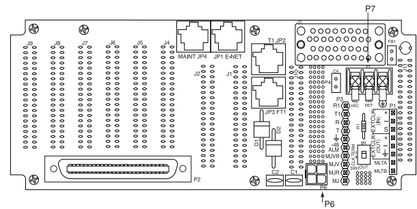
Figure 2. Total Access 850 Backplane
