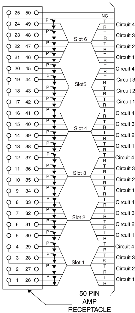
Figure 4. Connector Pinout
