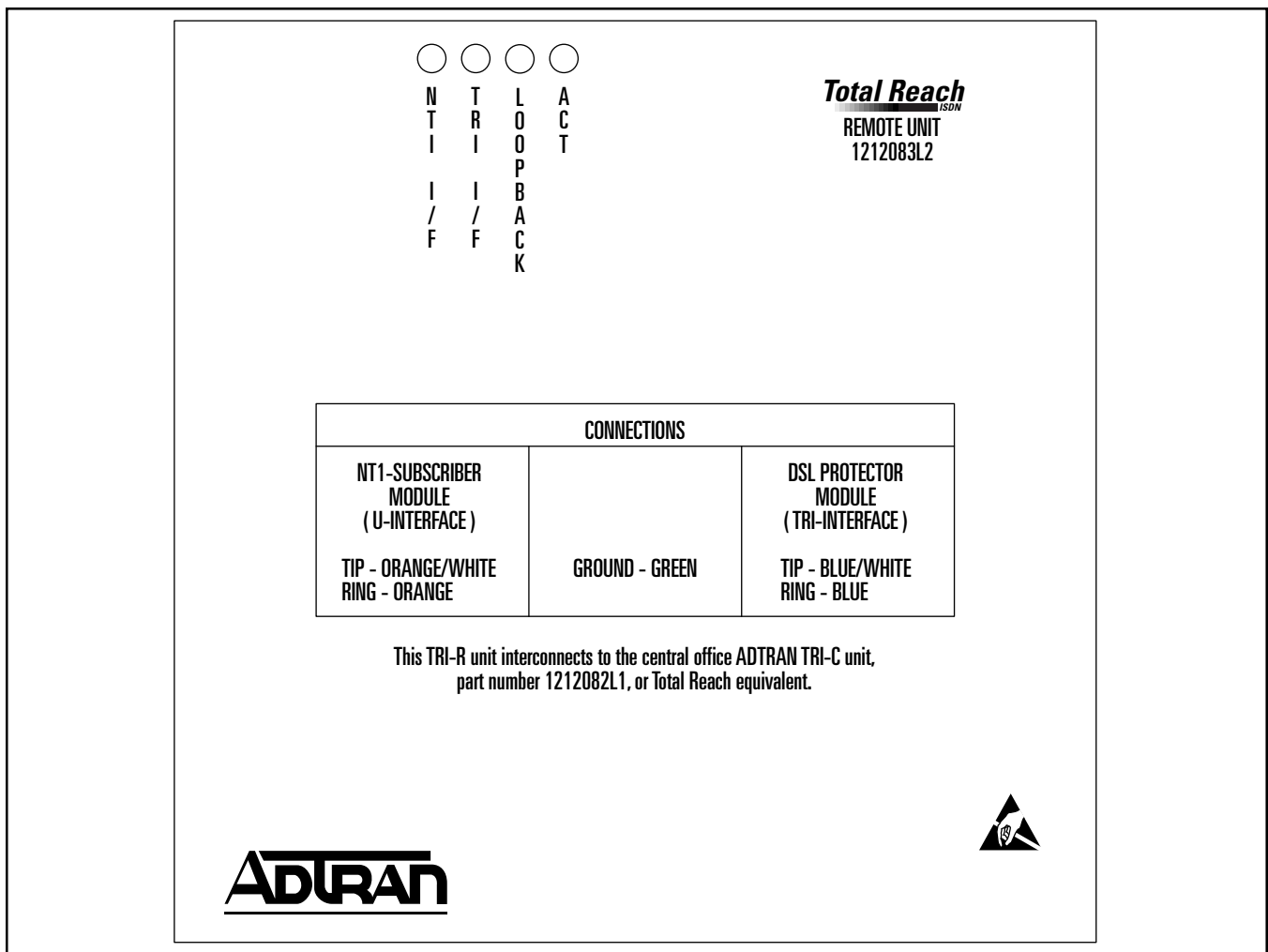
Figure 3. TRI-R/Encased Label
