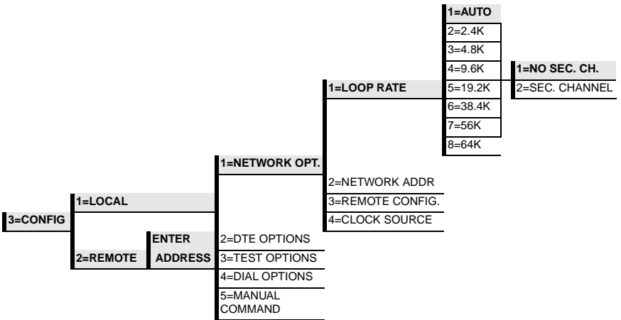
Figure 5-1. Setting Loop Rate Options
