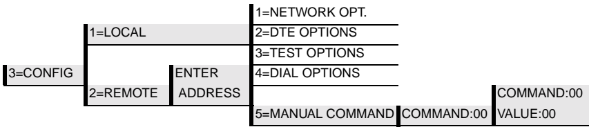
Figure 12-1. Manual Command
