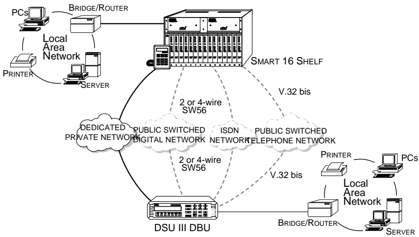
Figure 1-1. Typical Point-to-Point Application for DSU III DBU
