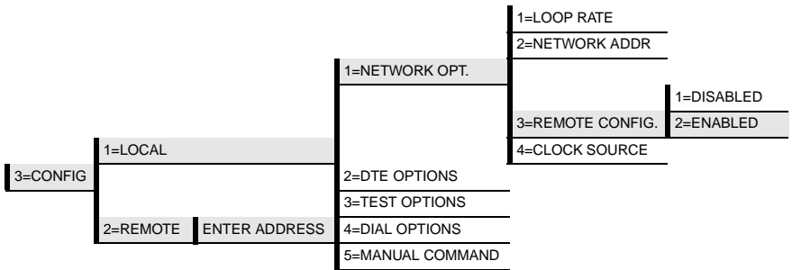
Figure 5-3. Remote Configuration
