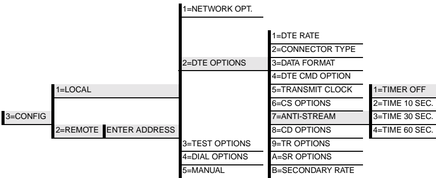
Figure 6-7. Anti-Stream Options
