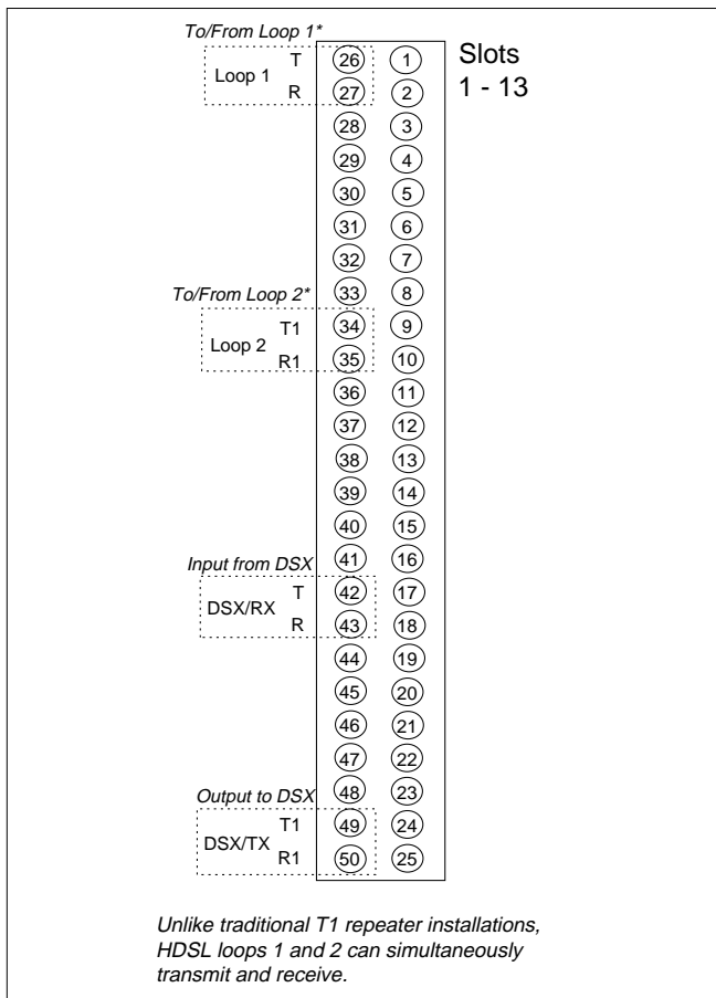
Figure 3. HTU-C Slot Wire Wrap Connections
