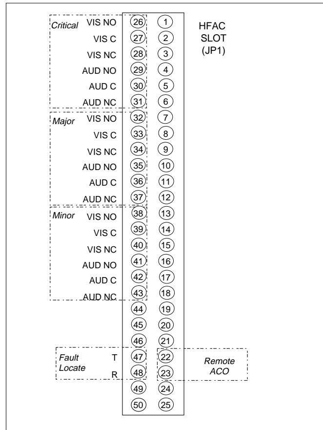
Figure 4. HFAC Controller Slot Wire Wrap Connections
