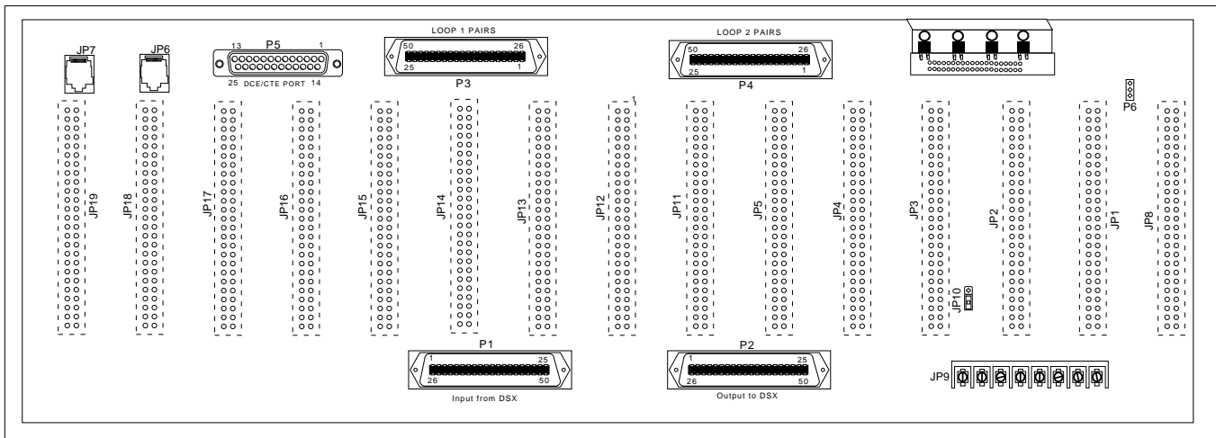
Figure 6. Signal I/O Connector Locations
