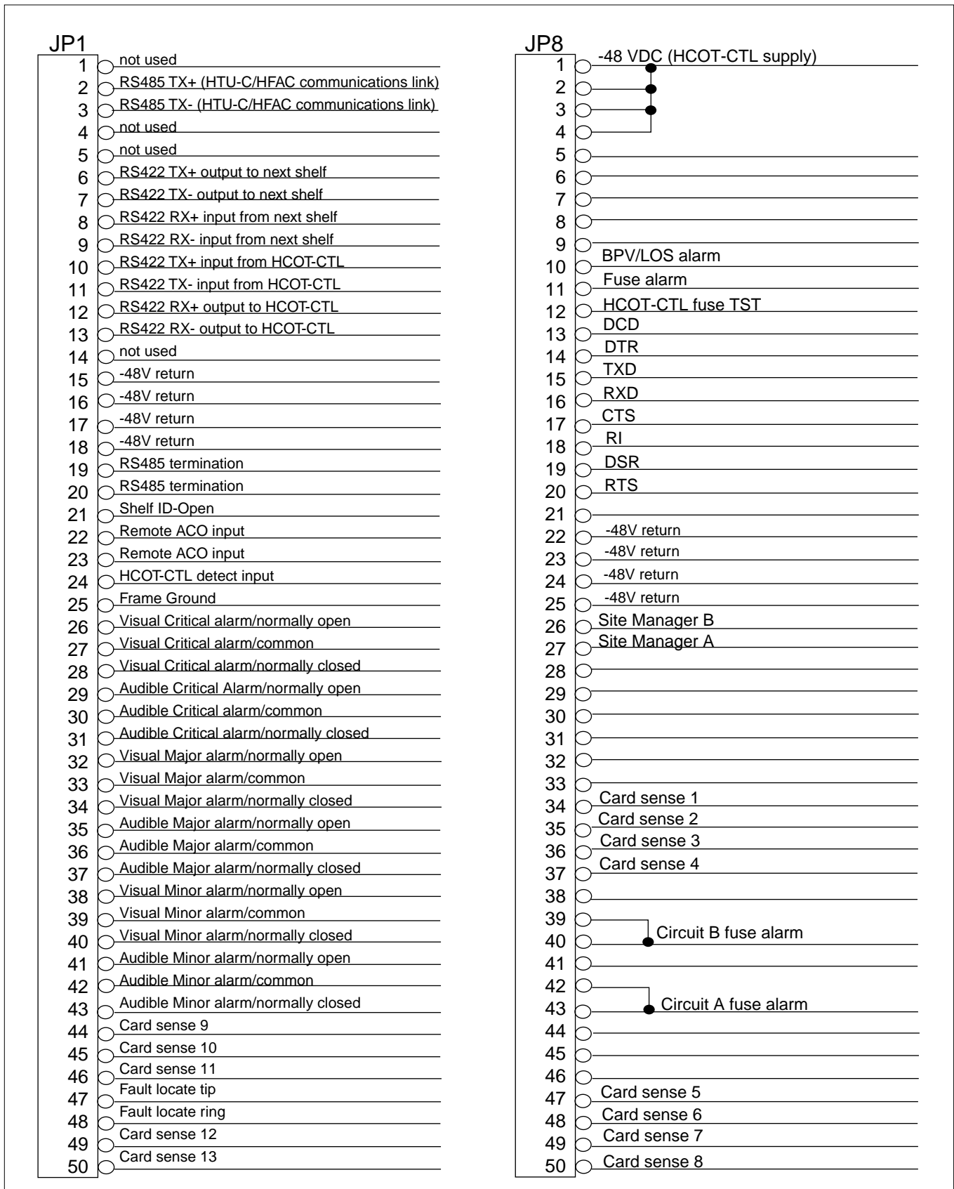
Figure 7. HFAC Slot Pin Assignments
