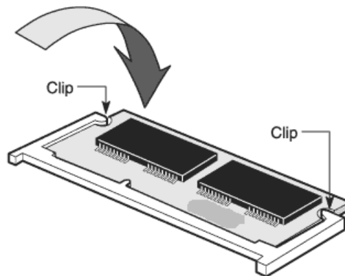
Figure 26. SODIMM Installation – Rotating the Module Downward
