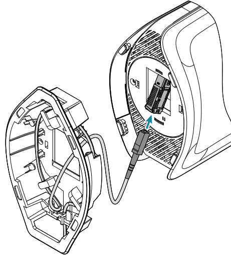
Figure 2. Connect the Fiber to the SDG Unit
