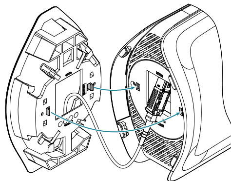
Figure 3. Align the Fiber Tray to the SDG Unit and Snap Into Place
