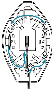
Figure 1. Wrap the Fiber Cable Counter-Clockwise in the Fiber Tray
